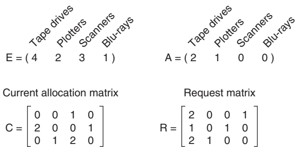
Figure 6-7. An example for the deadlock detection algorithm.
